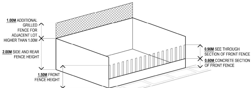
Figure 14. Fence Height
