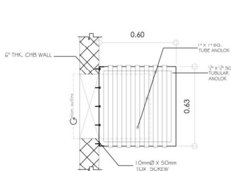
ELEVATION "B"
