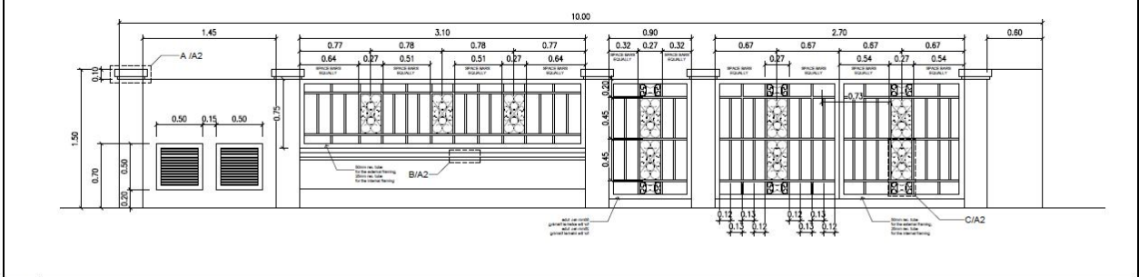
B FENCE ELEVATION A1 1:30M
