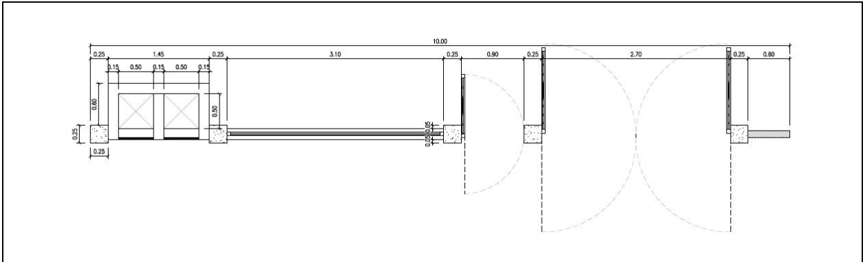
A FENCE PLAN 1:30M A1
