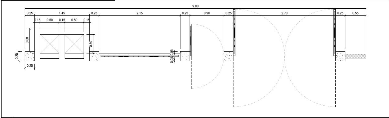
A FENCE PLAN 1:25M A1
