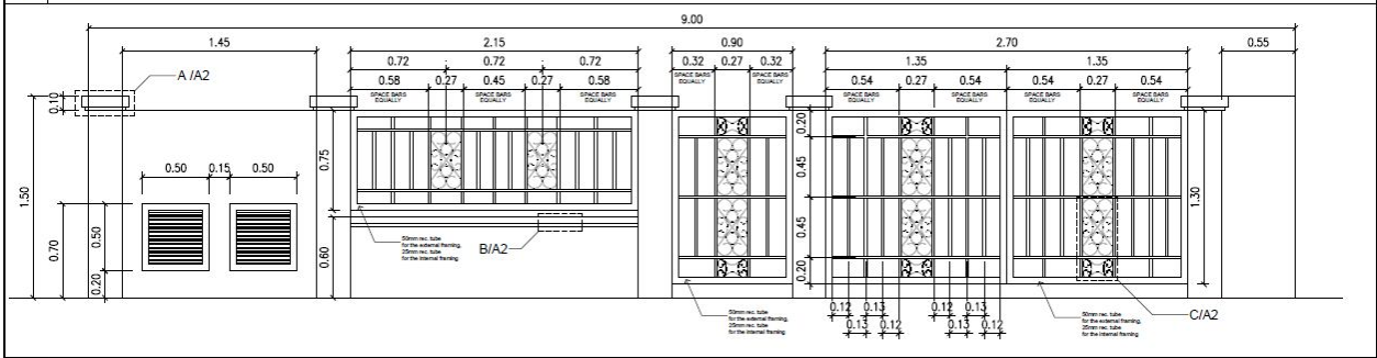
B FENCE ELEVATION A1 1:25M
